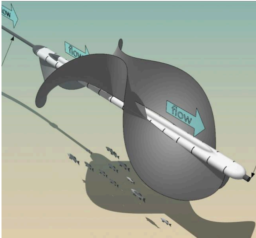
Short-tethered Traveling Wave Hydrokinetic (TWH) Pump by Pliant Energy
